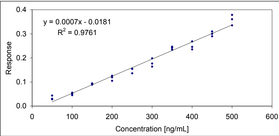
Figure 31: Calibration BDE197.
