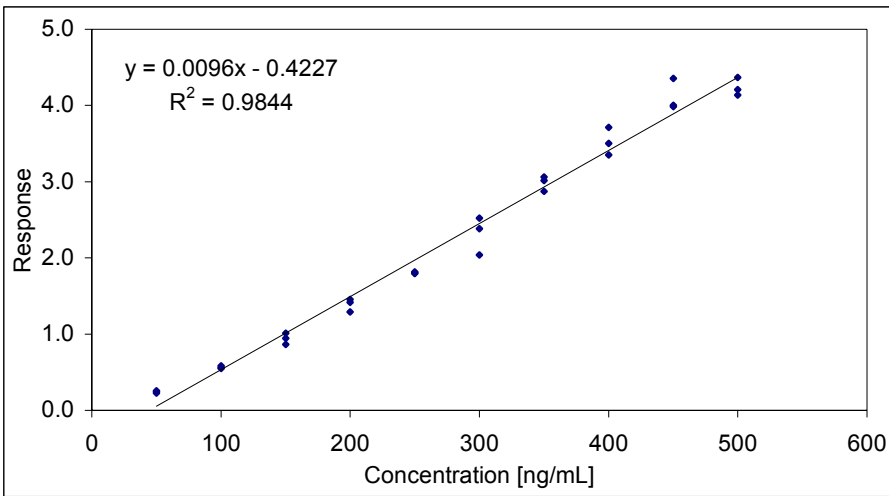
Figure 28: Calibration BDE100.
