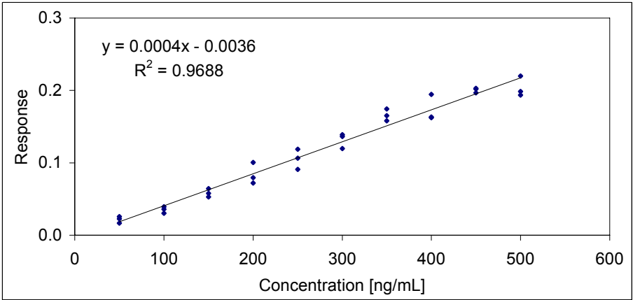
Figure 32: Calibration BDE203.
