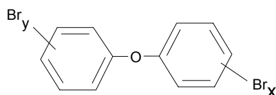
Figure 1: PBDE basic structure; \Sigma x,y : 1-10
