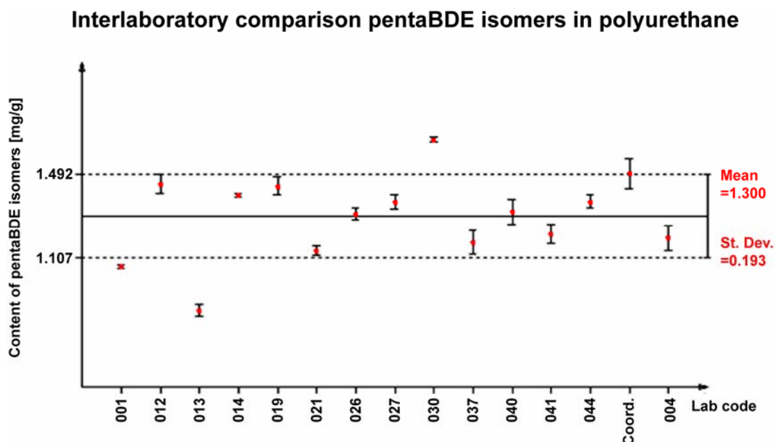
Figure 15: Graphical representation of the sum of pentaBDE isomers [mg g -1 ] in polyurethane with PENTA-BDE flame retardant (Mean: general mean; St. Dev: standard deviation); 15 laboratories (outliers expunged)
