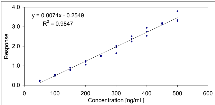
Figure 29: Calibration BDE99.
