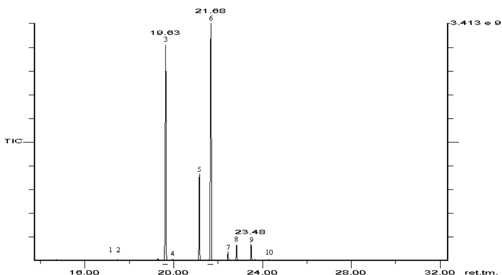
Figure 26: Chromatogram of technical PENTA-BDE; DB5-ms, 15 m, 0.25 mm ID, 0.1 µm df; 1 µL (50 ng/µL); 70°C (2 min) - 10°C/min - 300°C (15 min).
