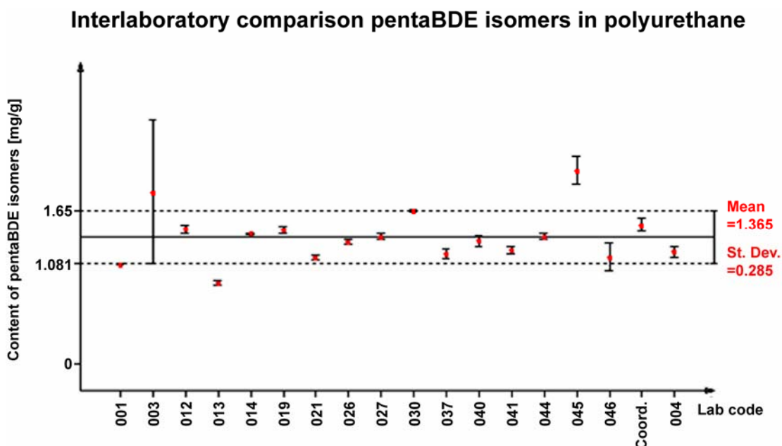
Figure 12: Graphical representation of the laboratory means as a sum of pentaBDE isomers [ \text{mg g}^{-1} ] in polyurethane with PENTA-BDE flame retardant (Mean: general mean; St. Dev: standard deviation); 18 laboratories.
