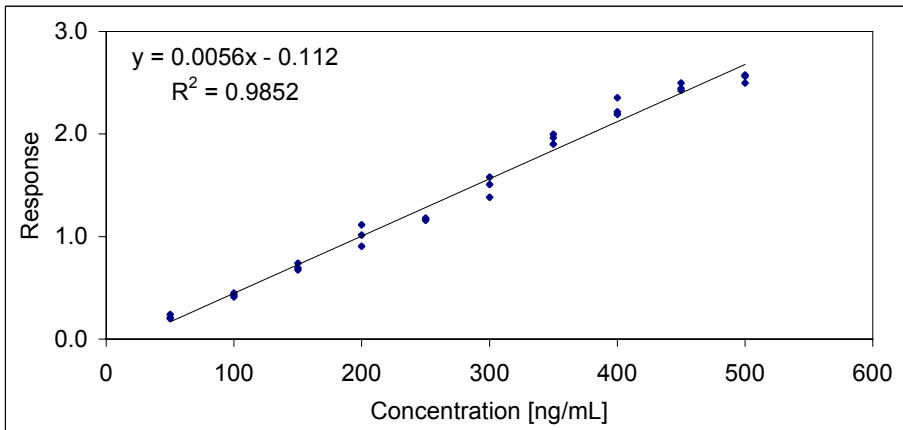
Figure 30: Calibration BDE85.
