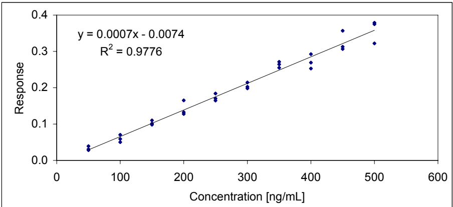
Figure 33: Calibration BDE196.
