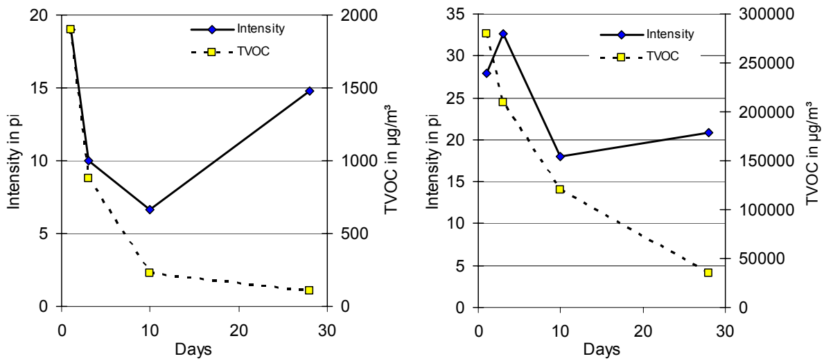
Figure 4-5: Odour intensity and TVOC of plasters 3342 (left) and 3345 (right)
