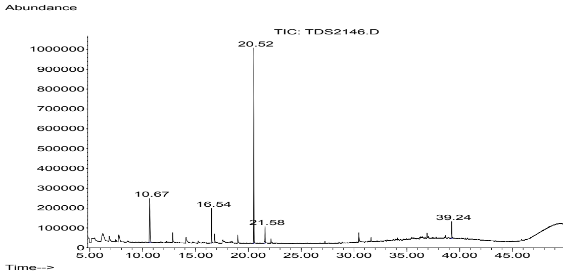
Figure 3461-1: GC/MS chromatogram on day 28 of emission testing on an adhesive for cork parquet on glass plate.
