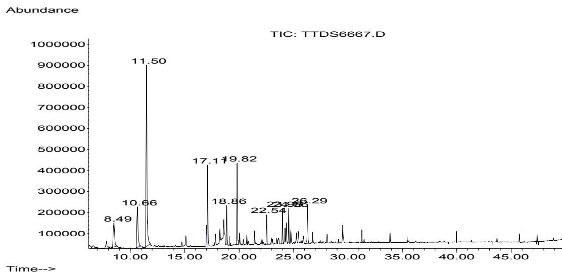
Figure 3382-1: GC/MS chromatogram on day 28 of emission testing on an OSB board.
