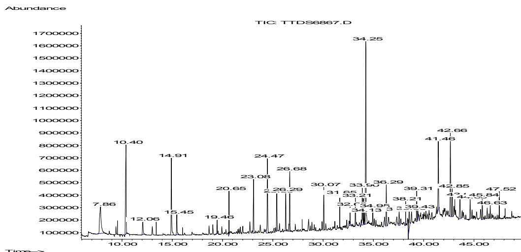
Figure 3332-1: GC/MS chromatogram on day 28 of emission testing on an acrylic sealant.
