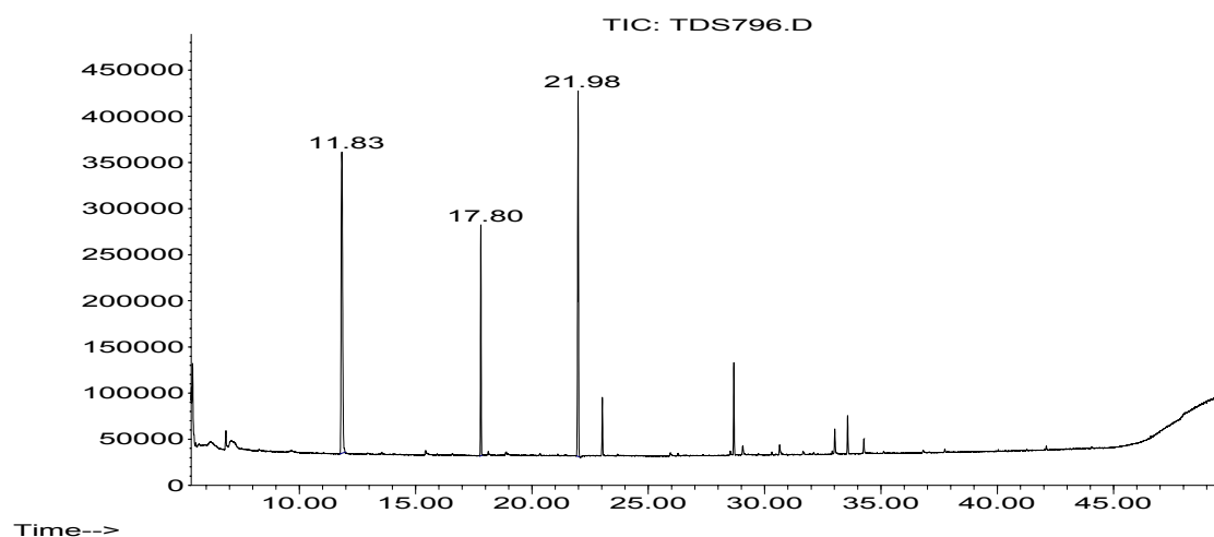
Figure 3463-1: GC/MS chromatogram on day 28 of emission testing on a dispersion wall paint on glass fibre non-woven fabric (3444) with adhesive (3445) on glass plate.
