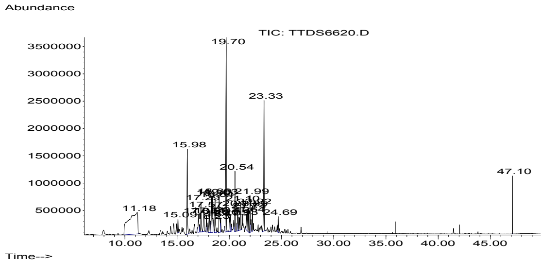
Figure 3351-1: GC/MS chromatogram on day 28 of emission testing on an acrylic sealant.
